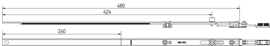
Extension lock 480 mm, 1 ML
