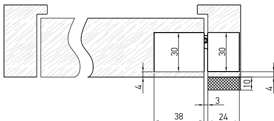
OPENED 90°
