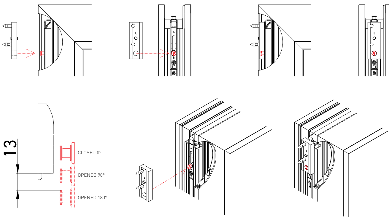
I7203-00-N03 Marking jig for locking plate
