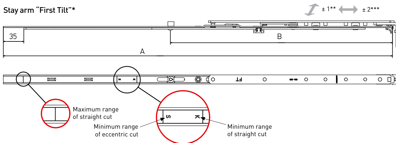
Stay arm "First Tilt"*, 1 MR
