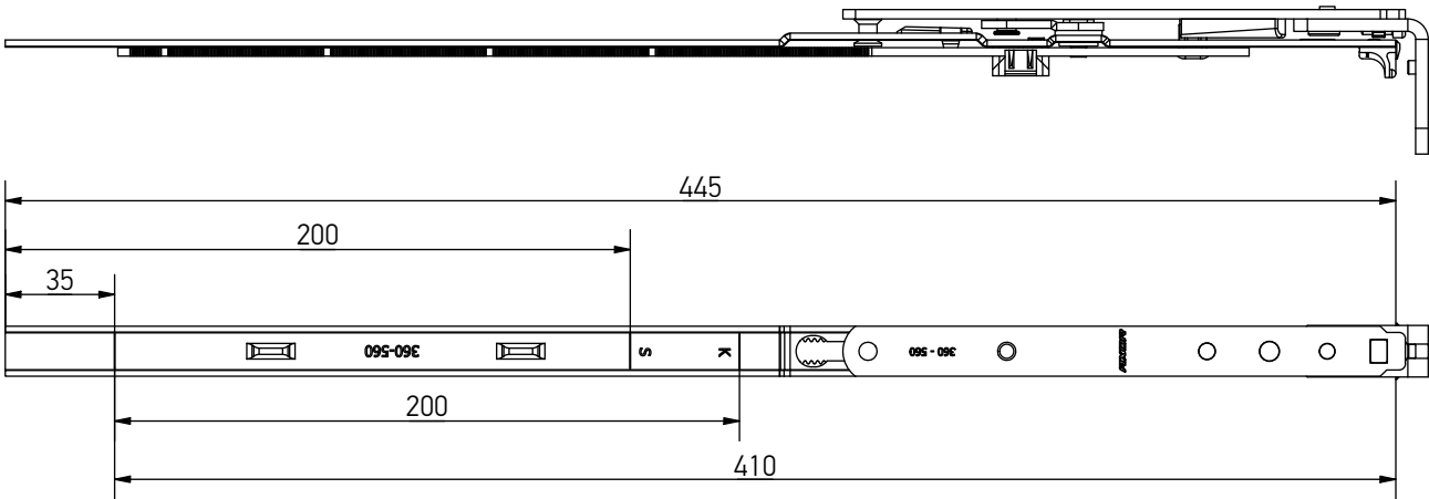
Stay arm
