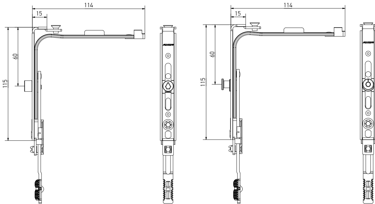
Narrow corner transmission, 1 ML, 15×115
