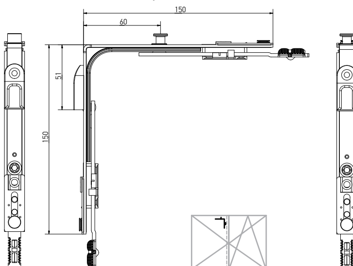
Corner transmission, double sash, 1 MR, 150×150, bottom
