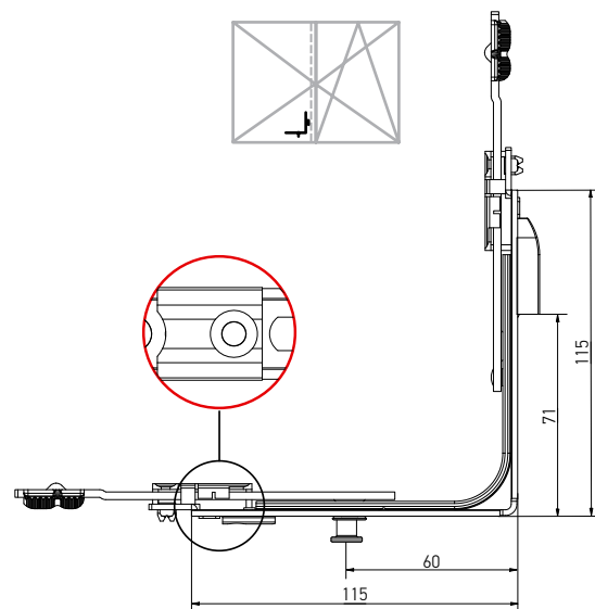
Corner transmission, double sash, 1 MR, 115×115, bottom
