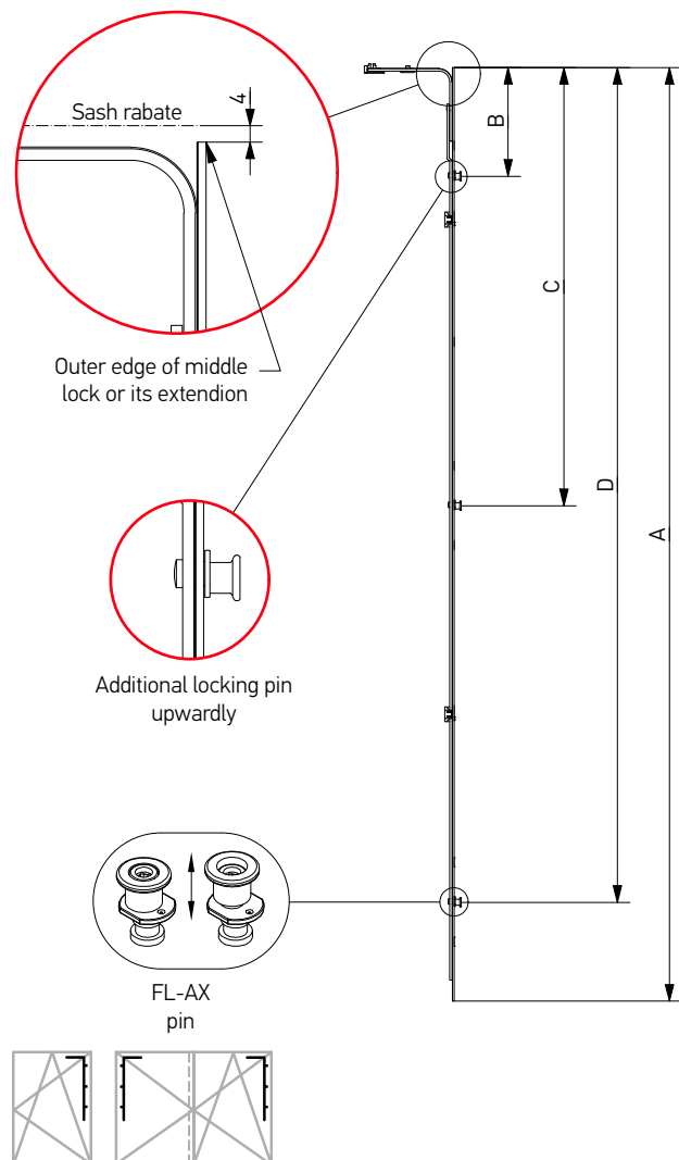
Middle lock ML with additional FL-AX pin
