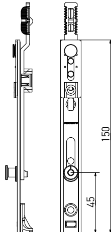
Bottom extension for turn sash 90° (bottom), 1 MR
