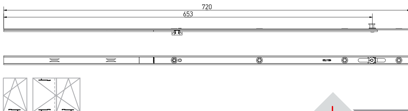
Extension lock 720 mm with possibility to cut, 1 MR
