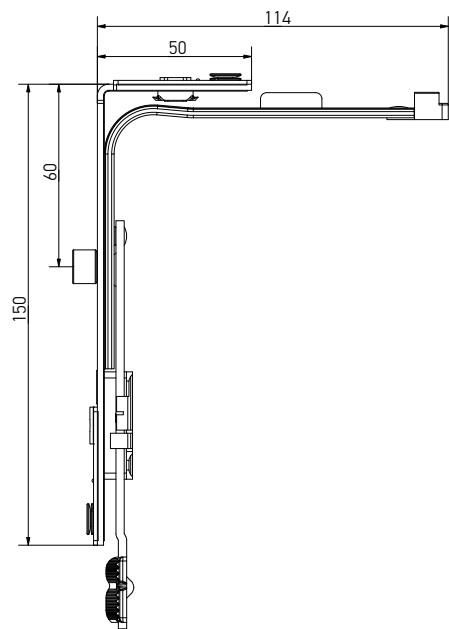
Narrow corner transmission, 1 ML, 50x150
