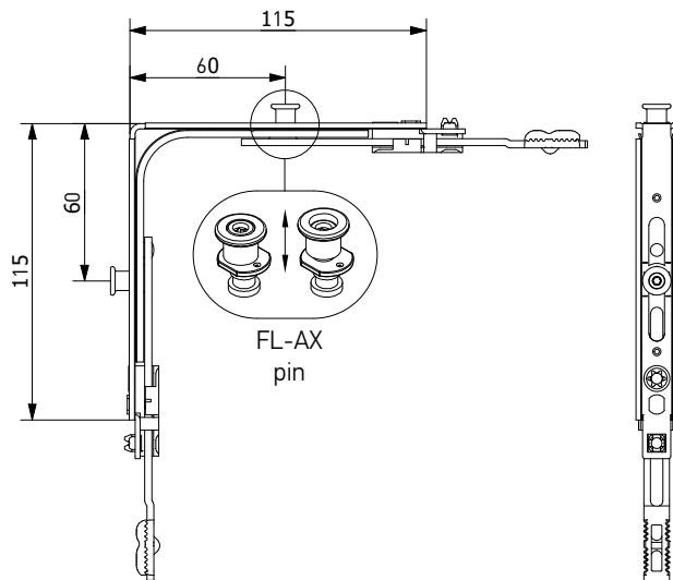
Corner transmission, bottom, 2FX
