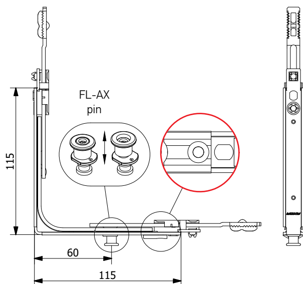
Corner transmission, bottom, 1FX
