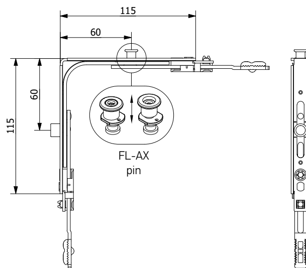
Corner transmission, bottom, 1FX +MAGNET
