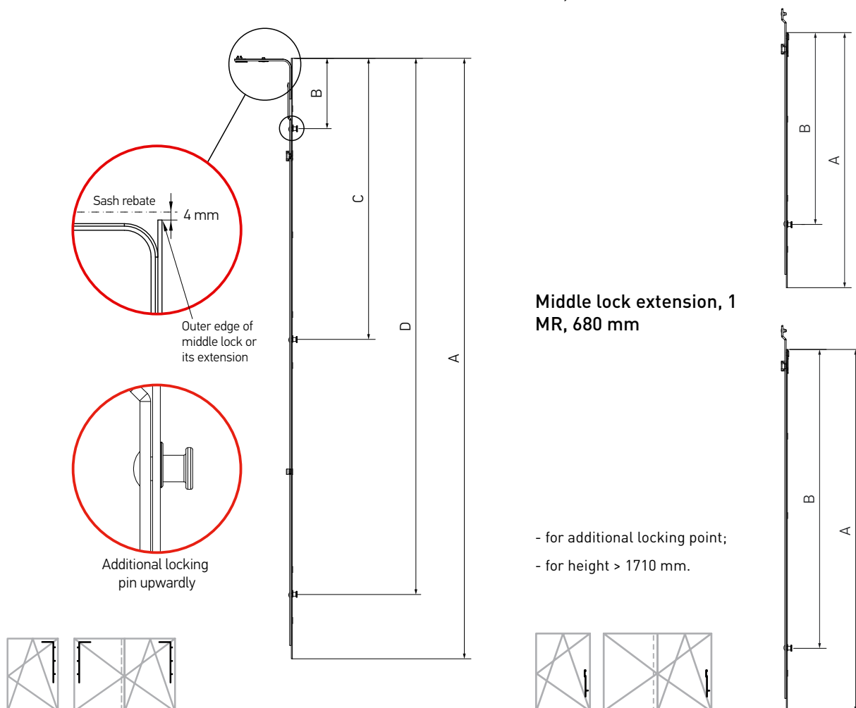
Middle lock extension, 1 MR, 480 mm
