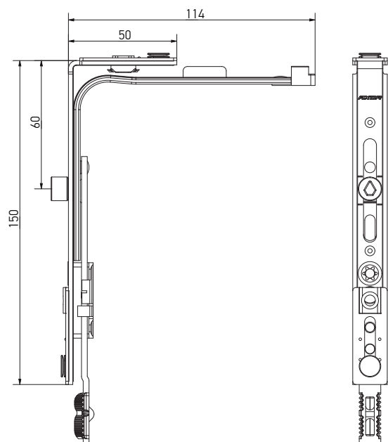
Narrow corner transmission, 1 ML, 50x150
