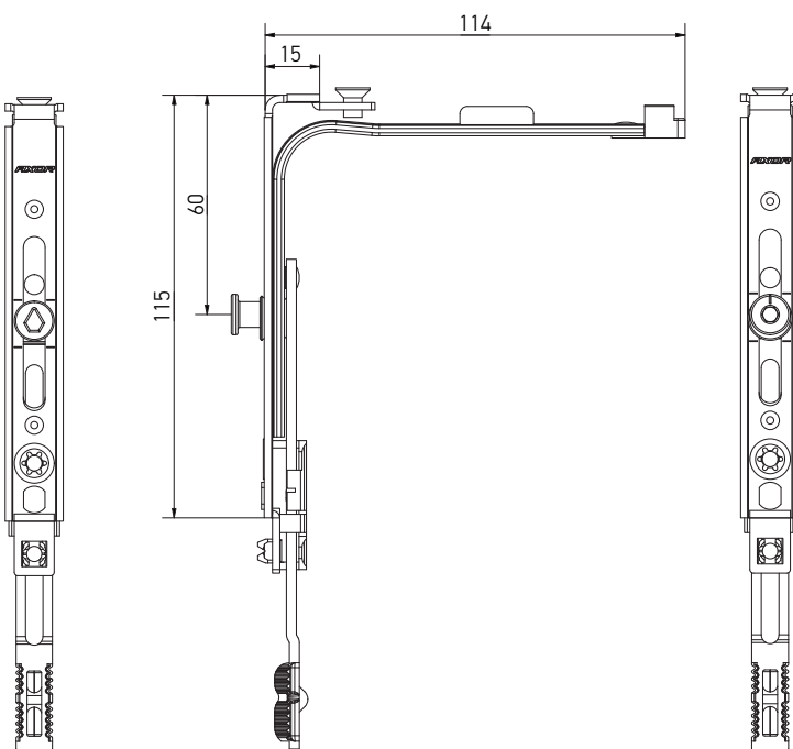
Narrow corner transmission, 1 MR, 115×15
