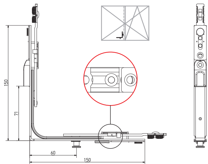
Corner transmission, double sash, 1 MR, 150×150, bottom
