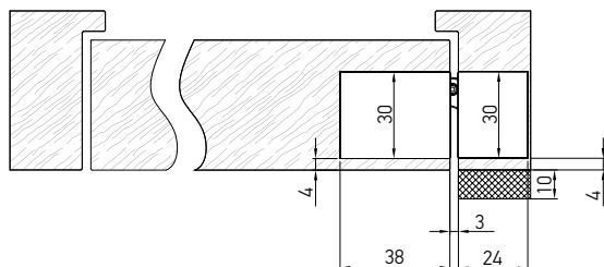
OPENED 90°
